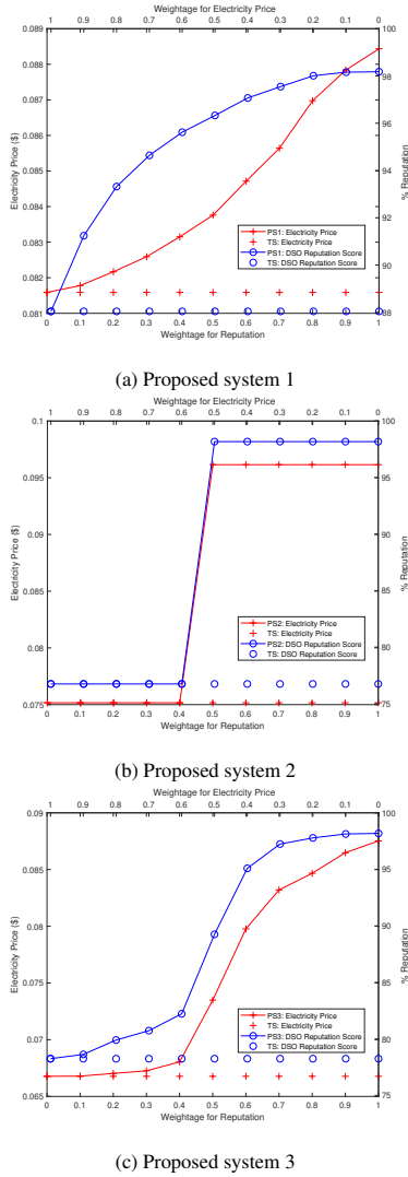
Figure 12: DSO selection mechanism
