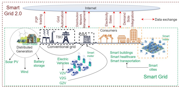
Figure 1: Smart Grid 2.0 architecture.
