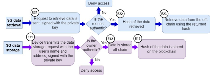
Figure 7: Deployment of energy data management service.
