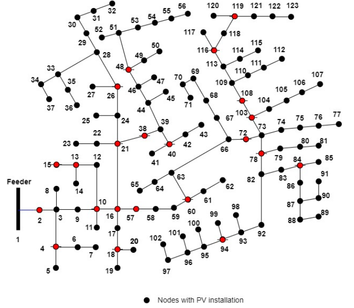
Figure 9: Modified IEEE 123 node distribution network
