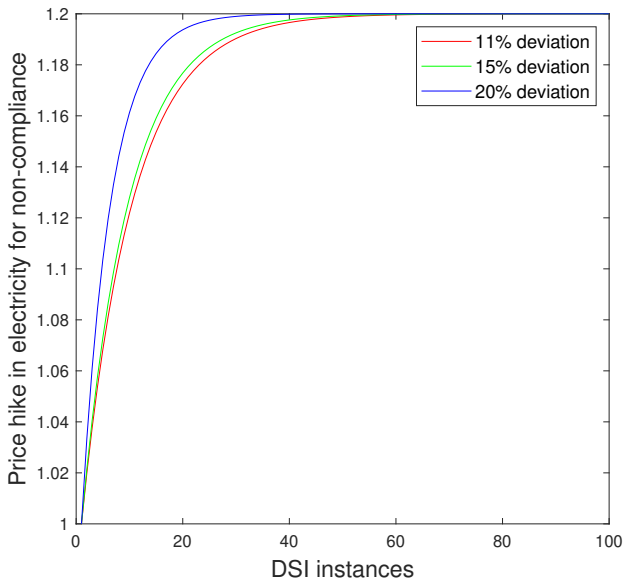
(b) Adjustment to the penalty received with deviation from DR signal
