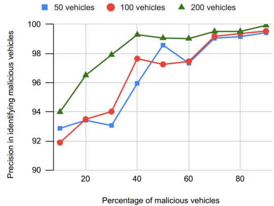
Fig. 4: Variation of precision with number of malicious vehicles
