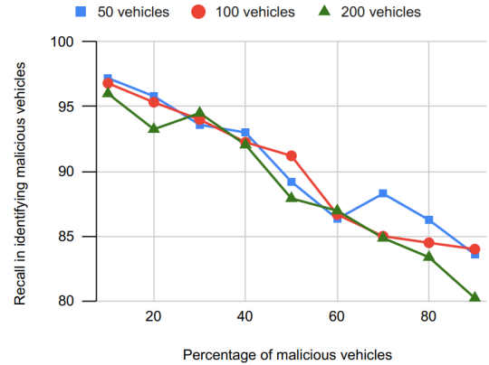
Fig. 3: Variation of recall with number of malicious vehicles
