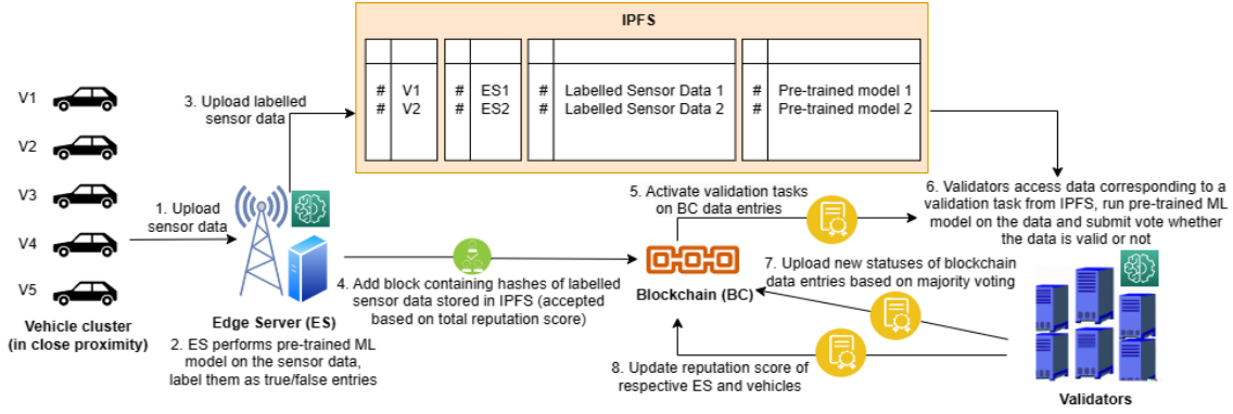
Fig. 1: Overview of the proposed solution for the IoV context
